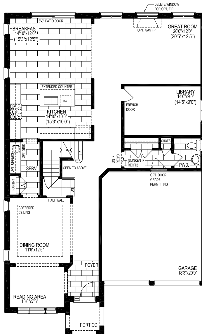
MAIN LEVEL STYLE A
