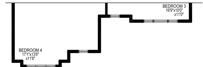
PART. SECOND LEVEL STYLE B
