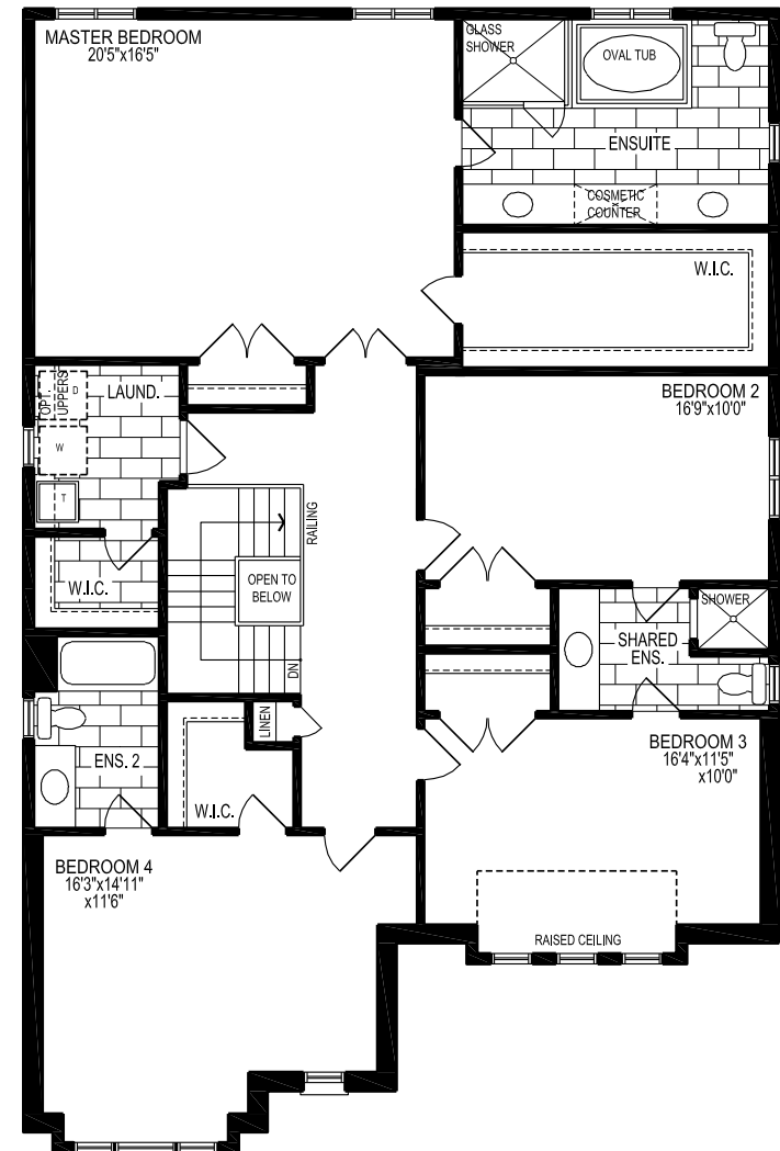
SECOND LEVEL STYLE A
