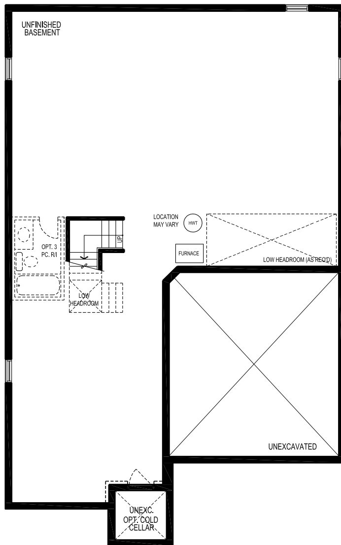
LOWER LEVEL STYLE A
